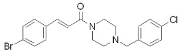
PC-6212701, CDCl 3
